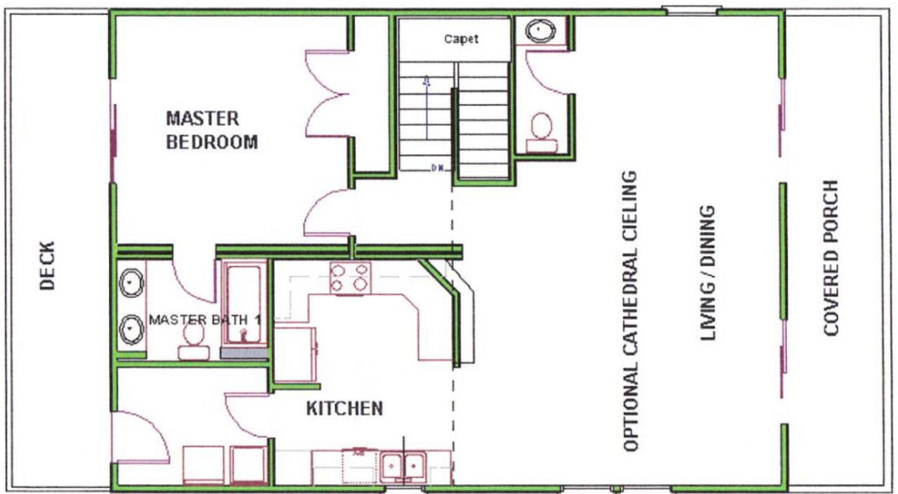
SECOND FLOOR
