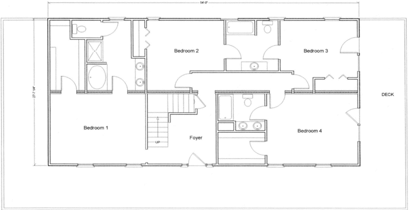
HUNTINGTON I FIRST FLOOR 1500 SF
