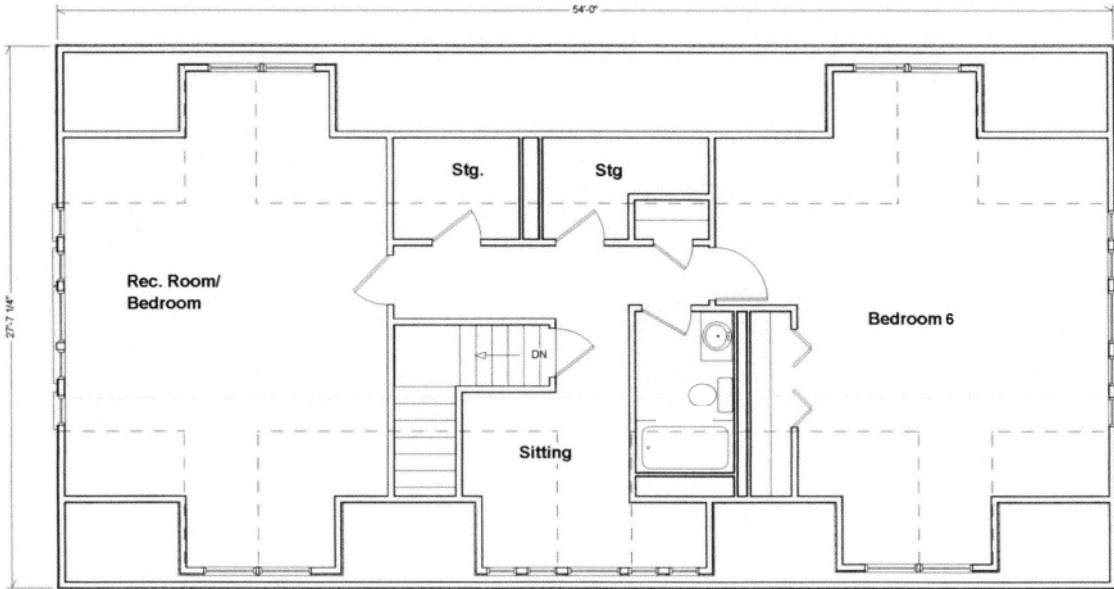
HUNTINGTON I THIRD FLOOR 975 SF
