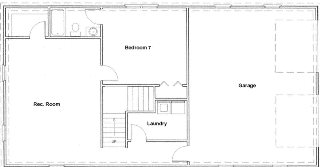
HUNTINGTON I OPTIONAL LOWER LEVEL 885 SF
