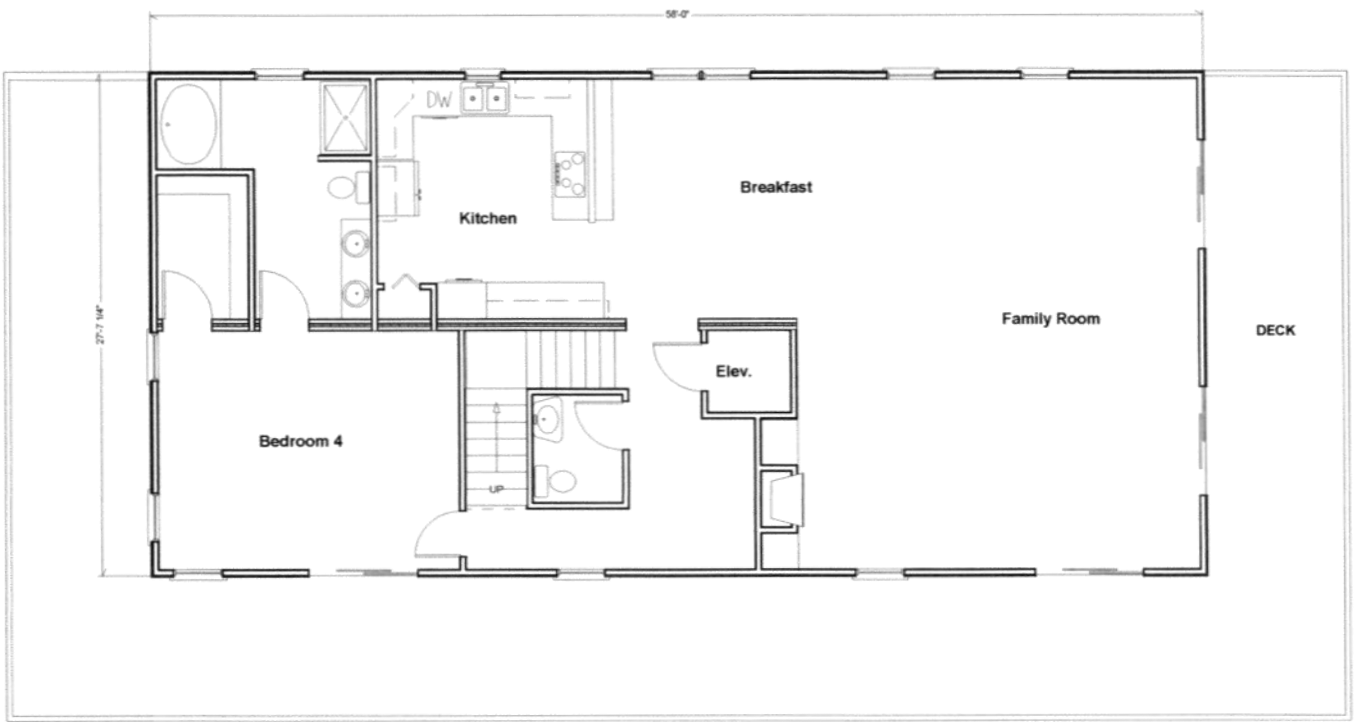
HUNTINGTON II SECOND FLOOR 1595 SF
